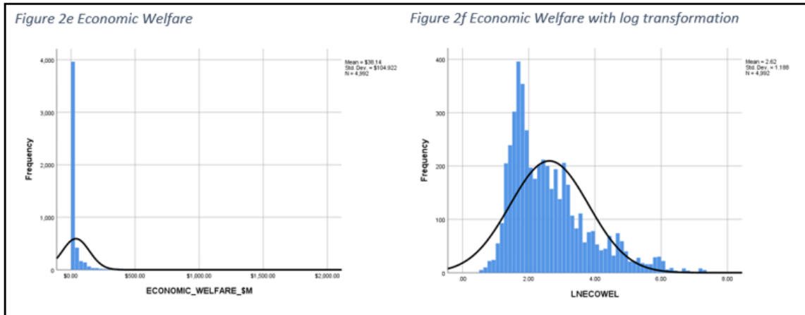
Figure 2. Histograms
